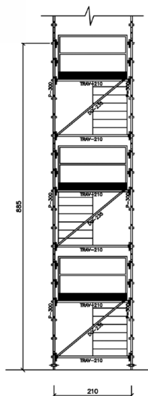
VISTA FRONTAL
